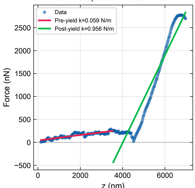
k80-linker1-paa-50nm-9000nm-10uN
