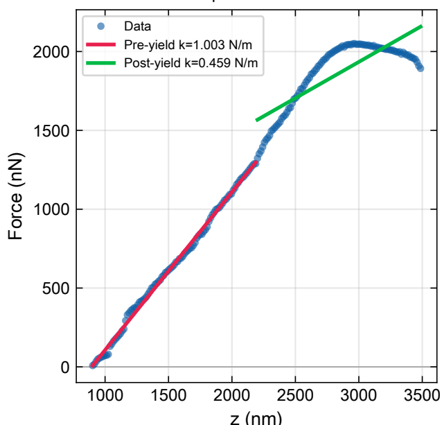
k80-linker1-paa-50nm-4500nm-3uN
