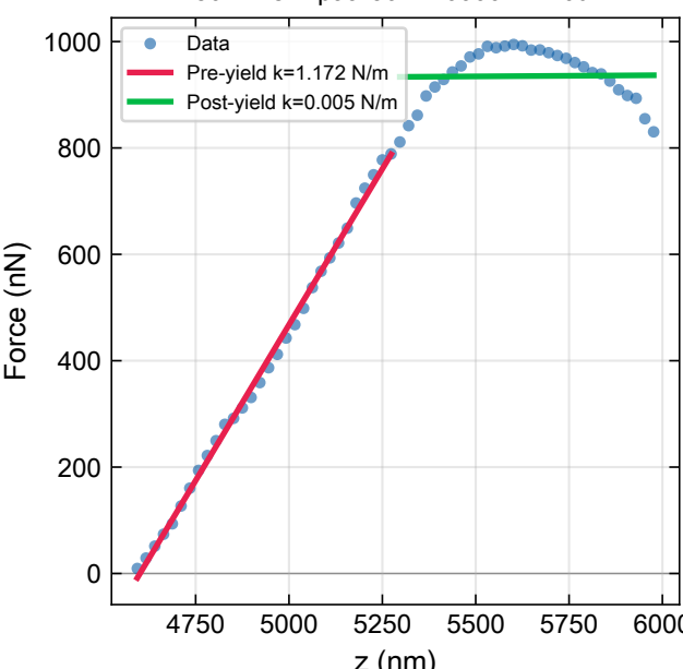
k80-linker1-paa-50nm-8000nm-10uN
