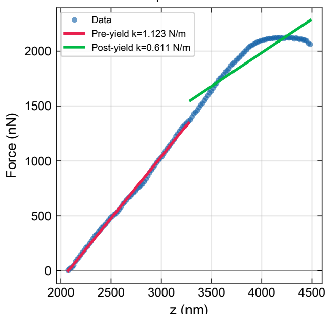
k80-linker1-paa-50nm-7000nm-10uN
