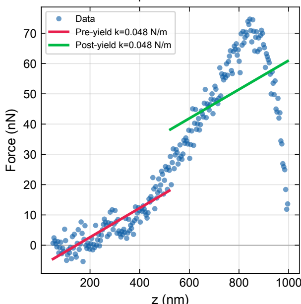
k80-linker1-paa-50nm-4000nm-3uN
