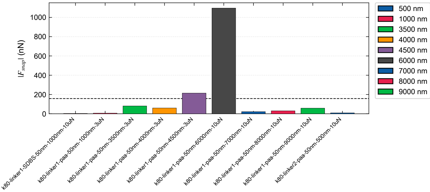
Snap-in Force Magnitude (All 10 Curves)
