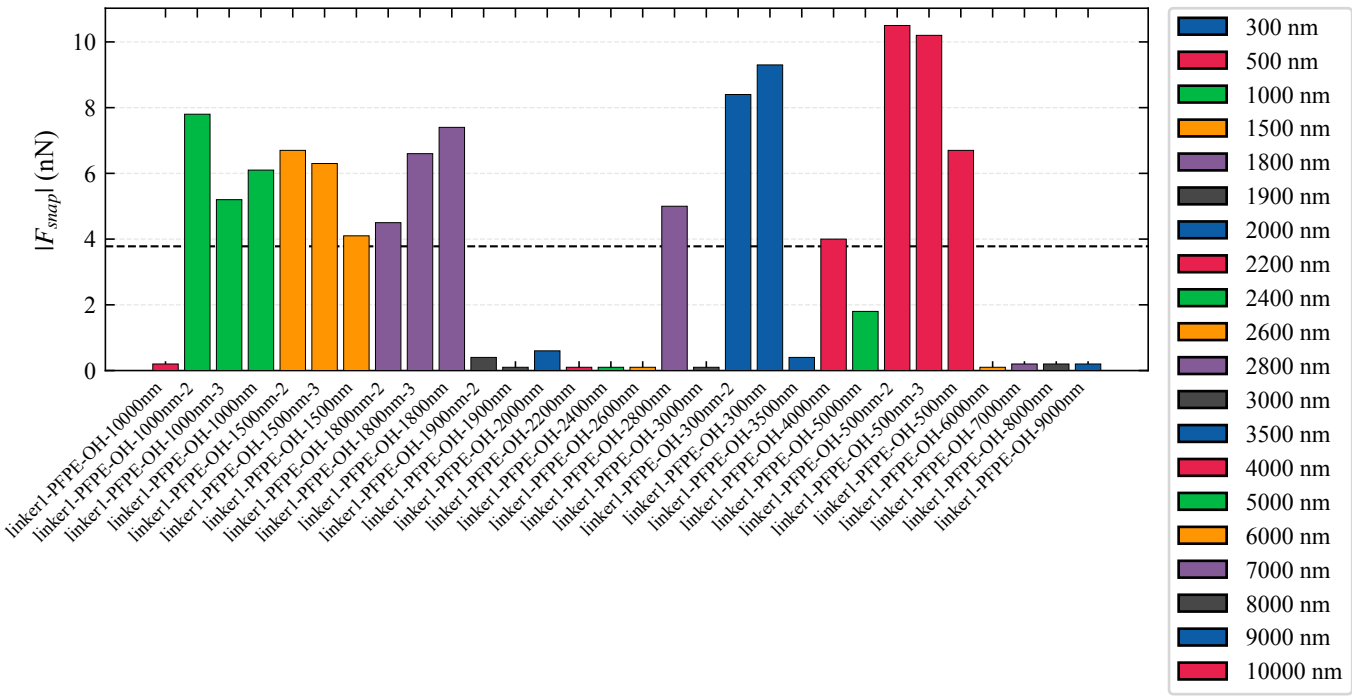
Snap-in Force Magnitude (All 30 Curves)
