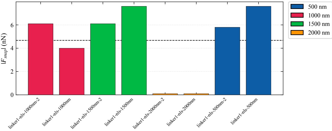
Snap-in Force Magnitude (All 8 Curves)
