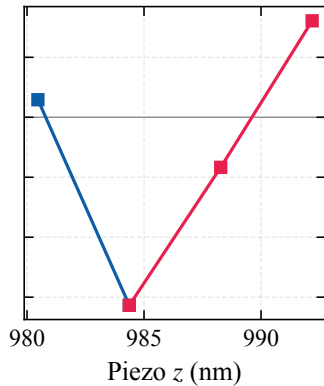
linker1-PFPE-OH-1000
