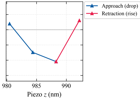
linker1-PFPE-OH-1000
