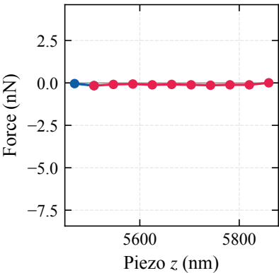
linker1-PFPE-OH-1000
