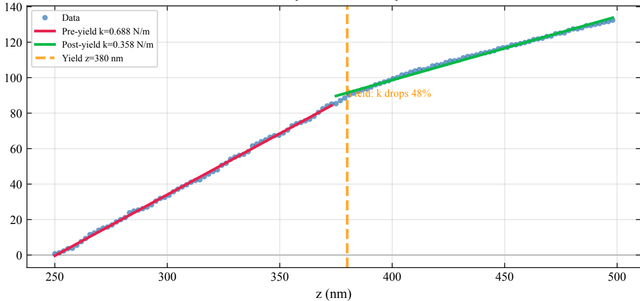
linker1-paa-100nN-500nm.spm
