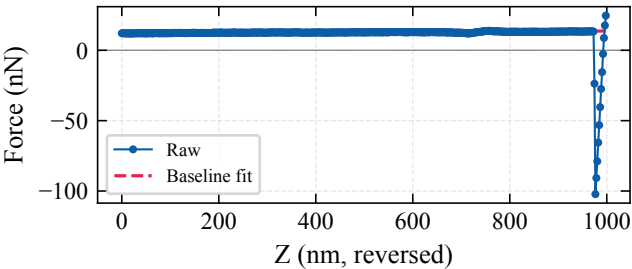
1000nm-10nN — Before correction
