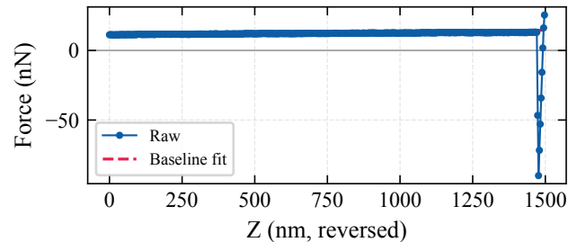
1500nm-9nN — Before correction
