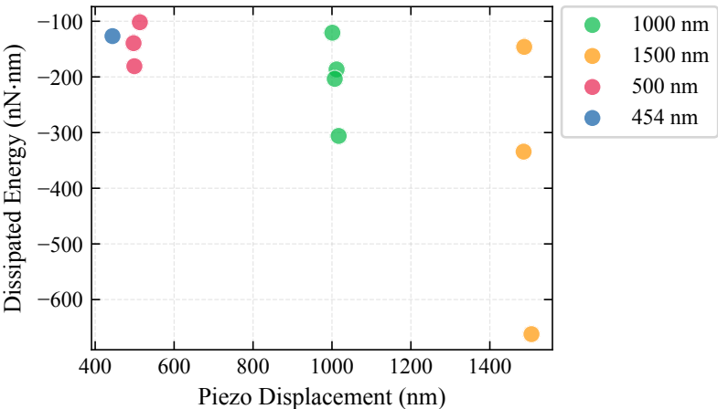
Energy Dissipated in Transition Zone
