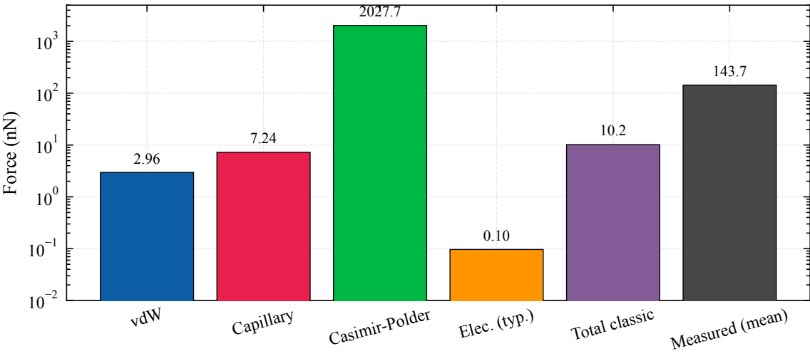
Theory vs. Measured Snap-in Force
