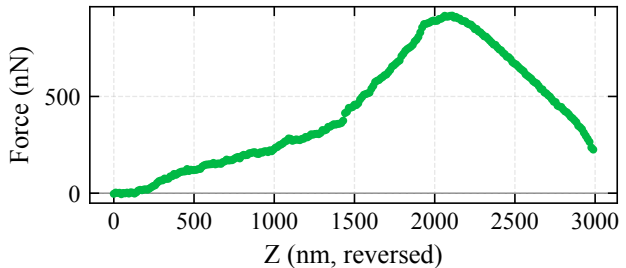
Slope=1.1050, Intercept=713.76 nN, N=9
