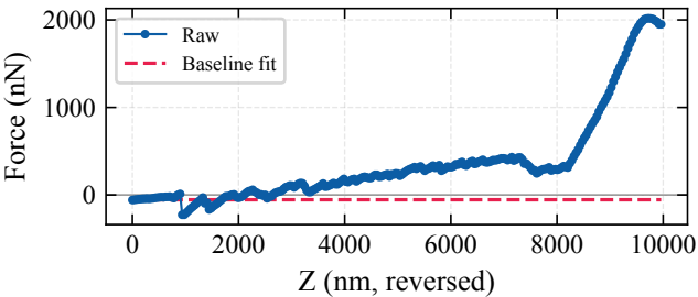
k80-linker1-paa-50nm-10000nm-1 — Before correction
