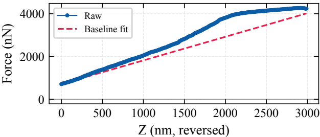
k80-linker1-paa-50nm-3000nm-3u — Before correction
