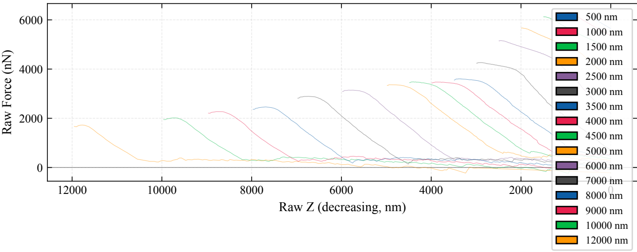
All 16 Raw Force-Distance Curves (Uncorrected, Overlay)
