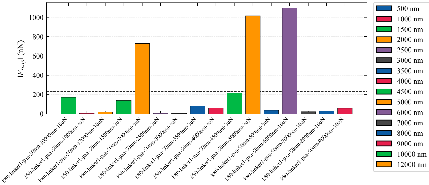
Snap-in Force Magnitude (All 16 Curves)
