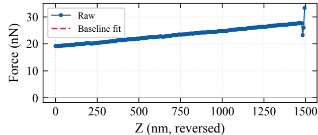
linker1-PFPE-OH-1500nm.spm — Before correction
