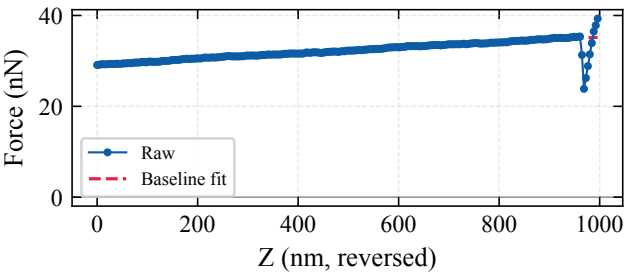
linker1-paa-1000nm-2.spm — Before correction
