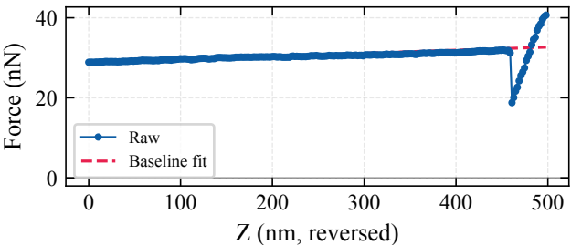
linker1-paa-500nm.spm — Before correction
