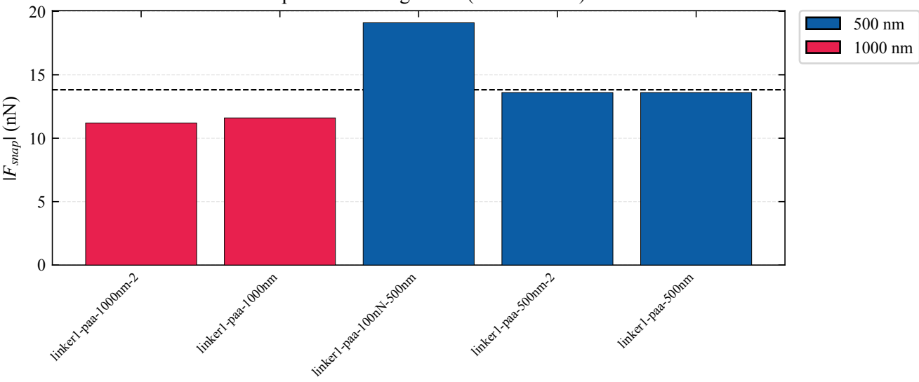
Snap-in Force Magnitude (All 5 Curves)
