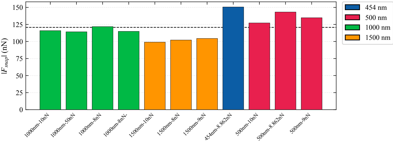
Snap-in Force Magnitude (All 11 Curves)
