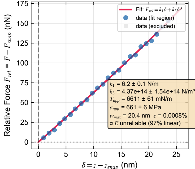
Bridge-arch membrane model fit
