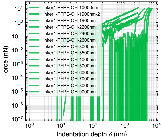
Force vs Indentation (log-log)
