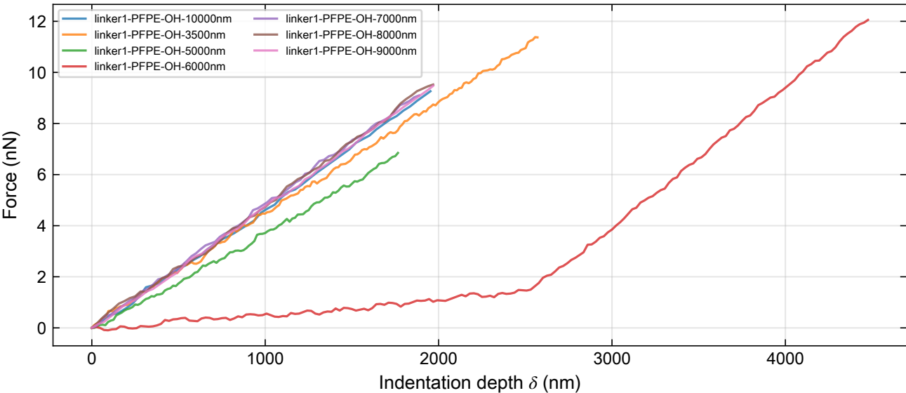
No-snap curves overlapped (N=7, origin = 5% max force)
