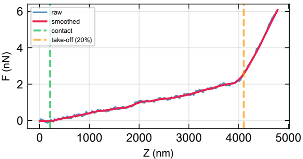
linker1-PFPE-OH-6000nm (no-snap)
