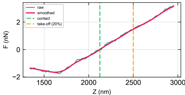
linker1-PFPE-OH-8000nm (no-snap)
