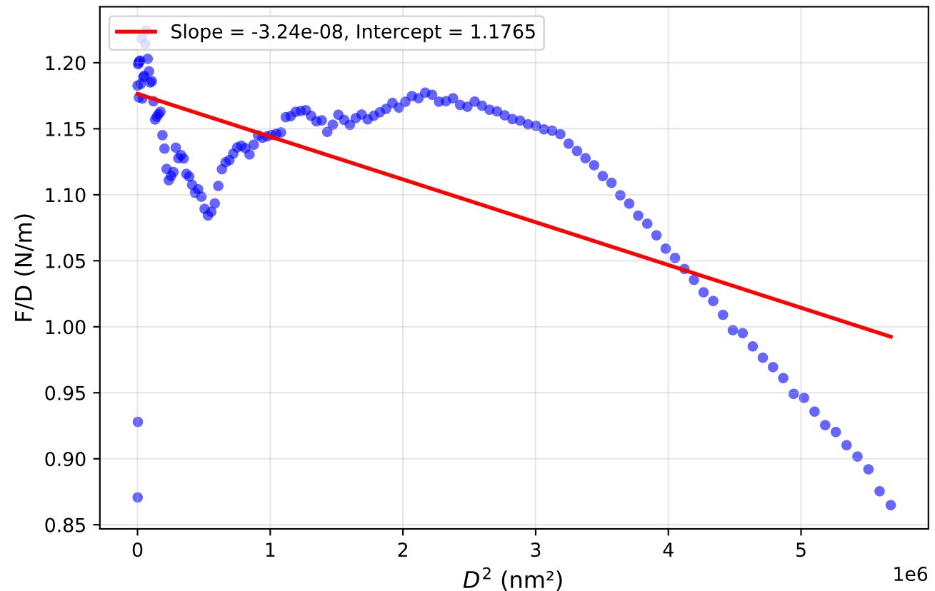
linker1 - Linearized: F/D = k_1 + k_3 D^2
