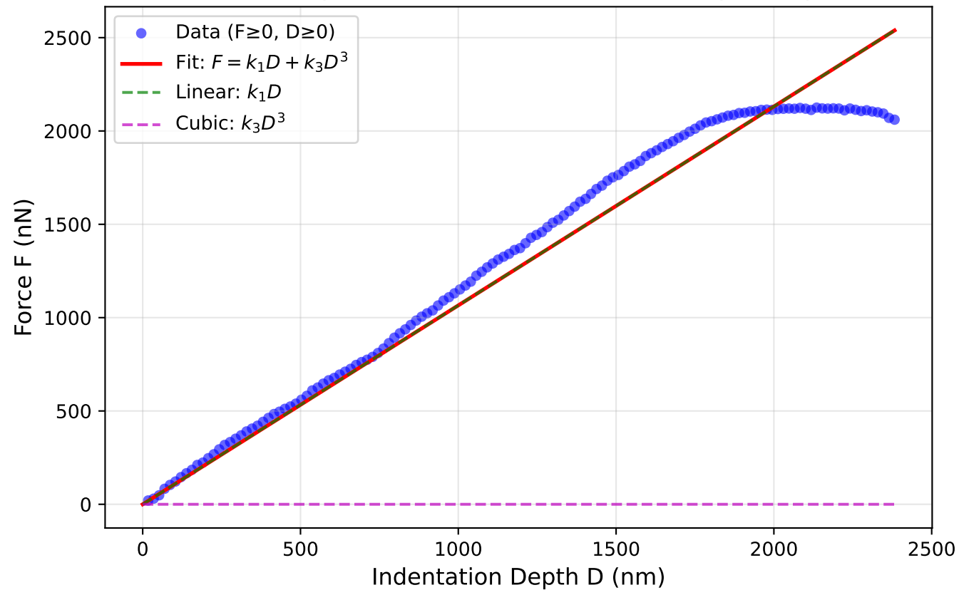
linker1 - Best Fit ( R^2 = 0.961 ) k80-linker1-paa-50nm-4500nm-3uN - NanoScope Analys...
