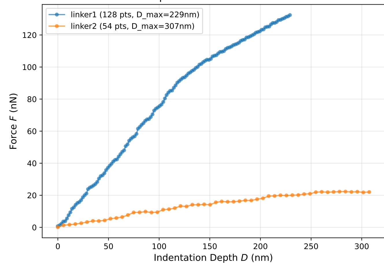
Representative F-D Curves
