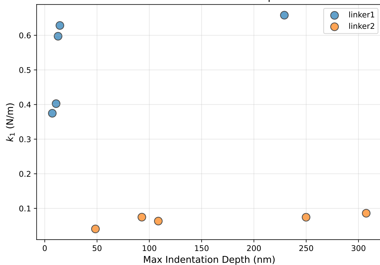
Linear Stiffness vs Max Depth
