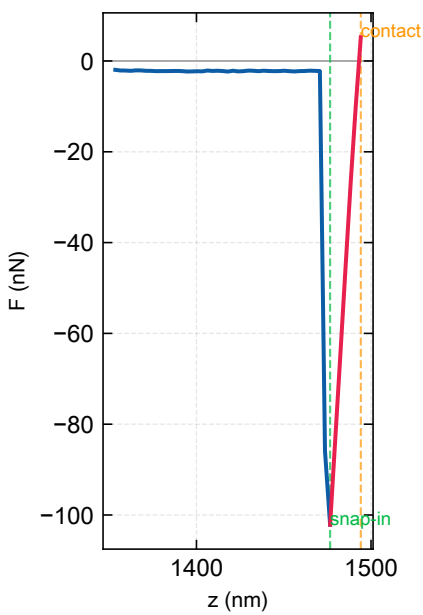
JJS-50nm-1500nm-8nN
