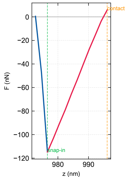
JJS-50nm-454nm-8.862nN
