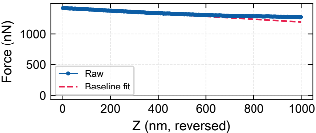
k80-linker1-SDBS-50nm-1000nm-1 — Before correction
