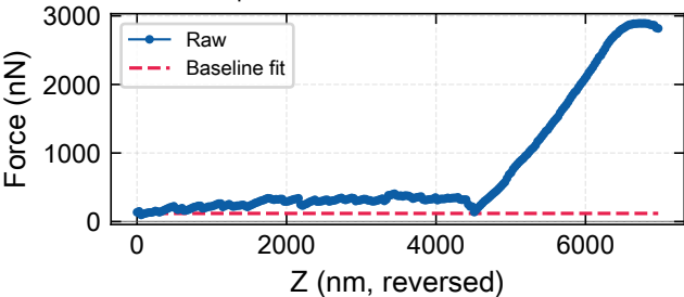
k80-linker1-paa-50nm-7000nm-10 — Before correction
