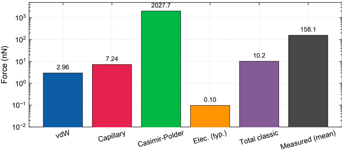
Theory vs. Measured Snap-in Force
