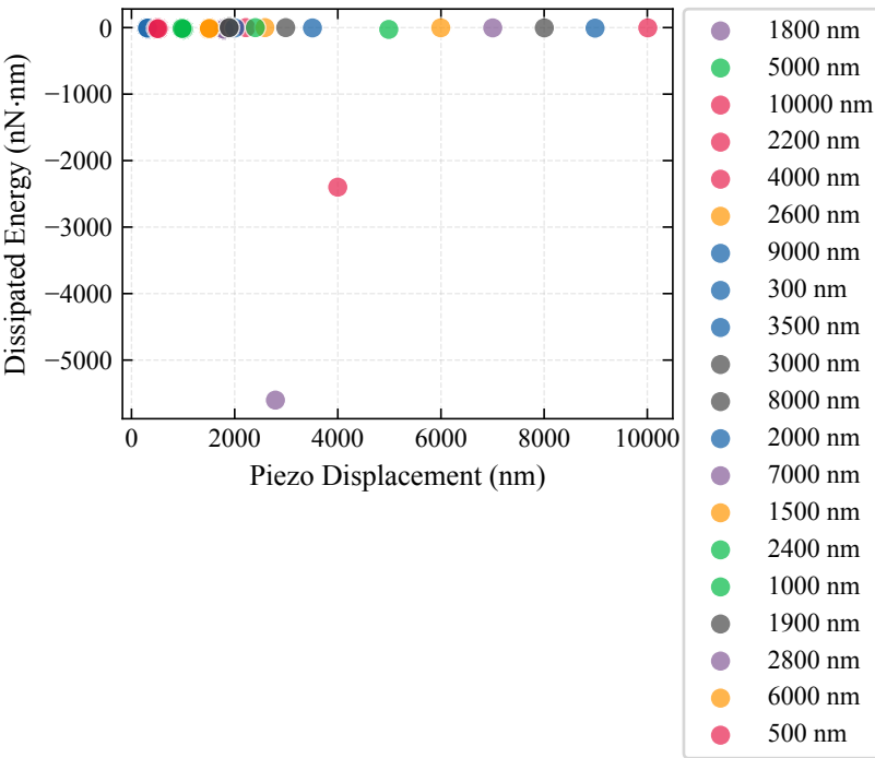
Energy Dissipated in Transition Zone
