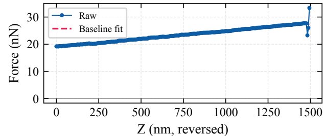
linker1-PFPE-OH-1500nm.spm — Before correction
