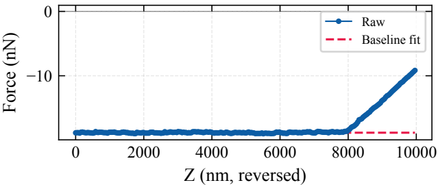
linker1-PFPE-OH-10000nm.spm — Before correction
