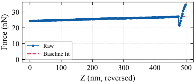
linker1-nls-500nm-2.spm — Before correction
