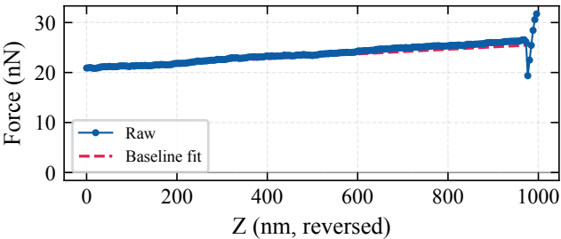
linker1-nls-1000nm-2.spm — Before correction
