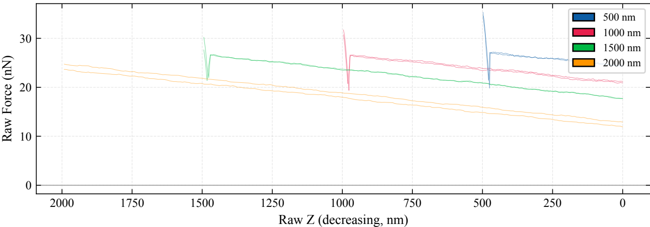
All 8 Raw Force-Distance Curves (Uncorrected, Overlay)
