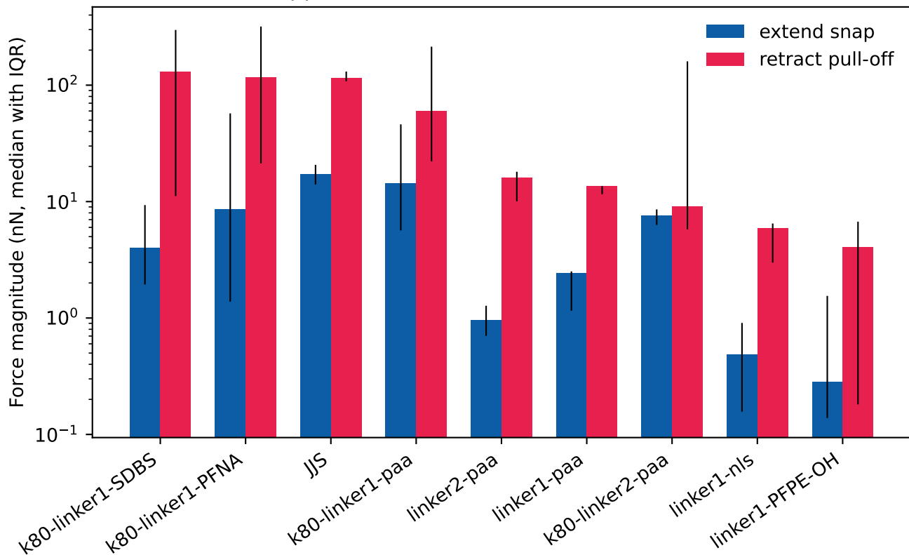
Approach attraction vs. retract adhesion
