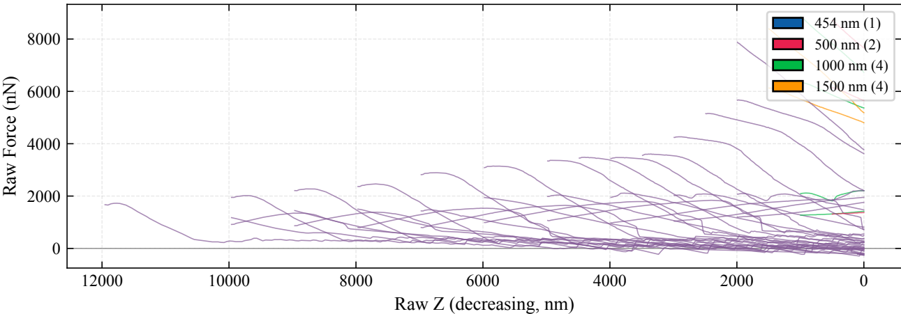
All 11 Raw Force-Distance Curves (Uncorrected)
