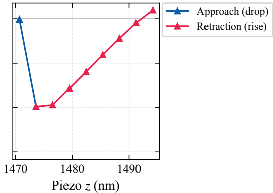
1500 nm / 10 nN
