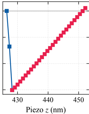
454 nm / 8.862 nN
