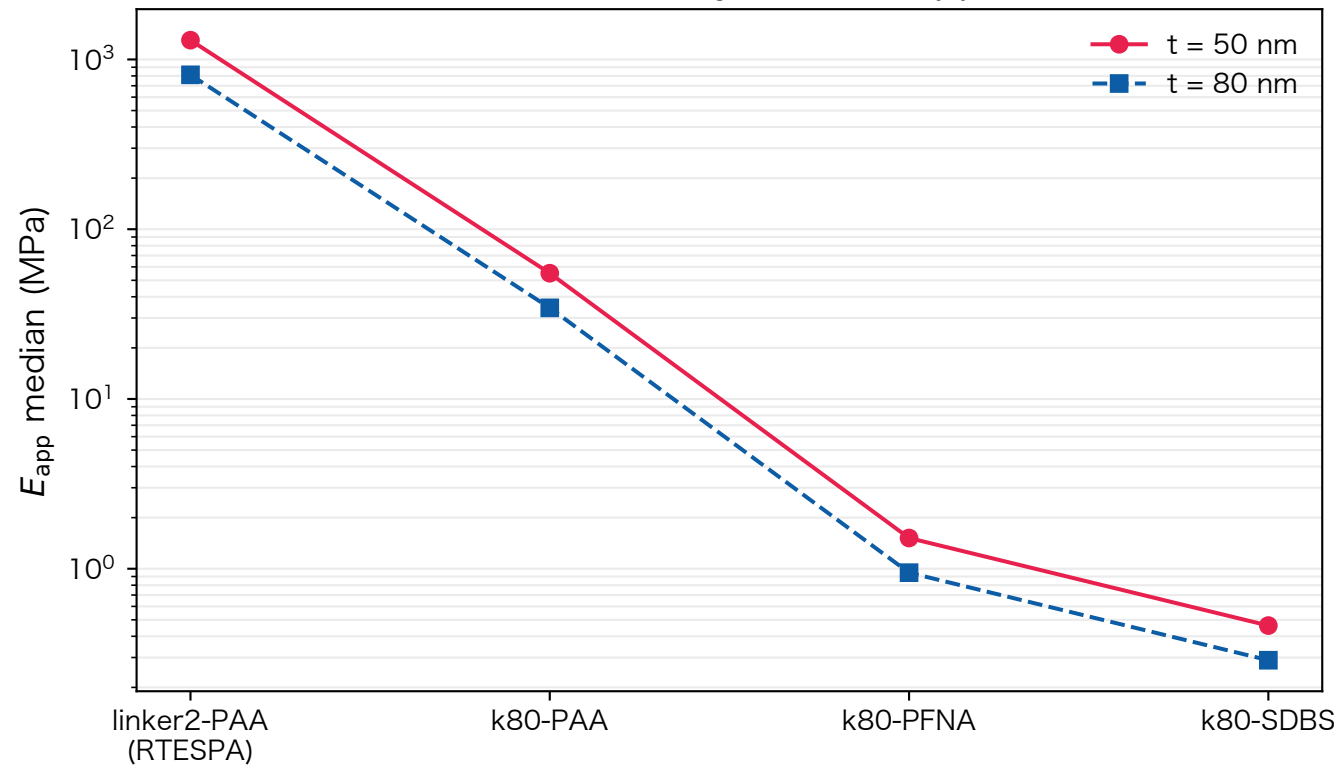
Thickness sensitivity follows E_{app} \propto 1/t
