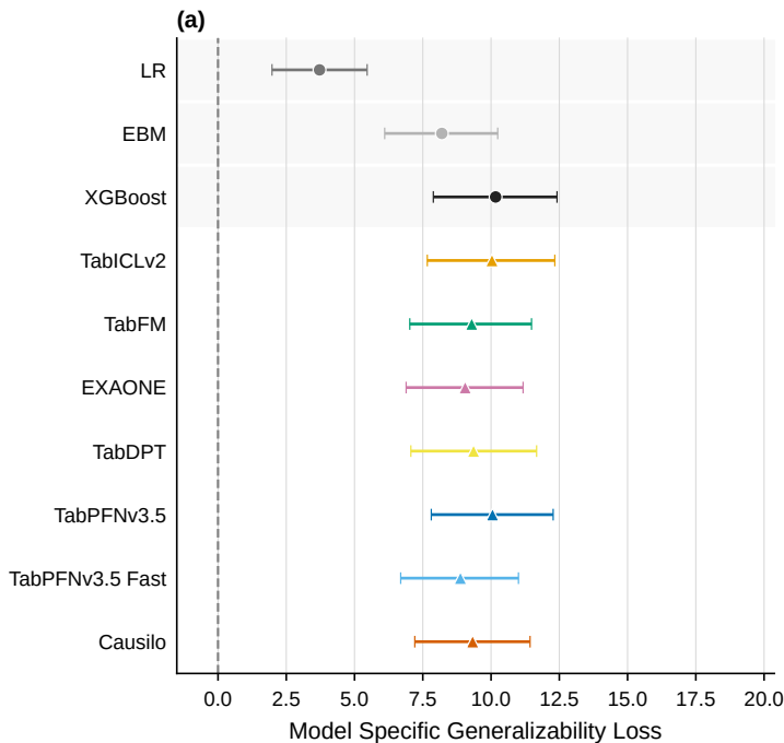
Evaluation: MIMIC-IV
