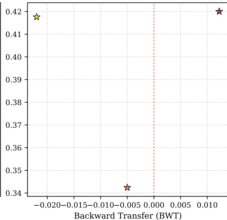
(c) Sweep C: split-CIFAR-100
