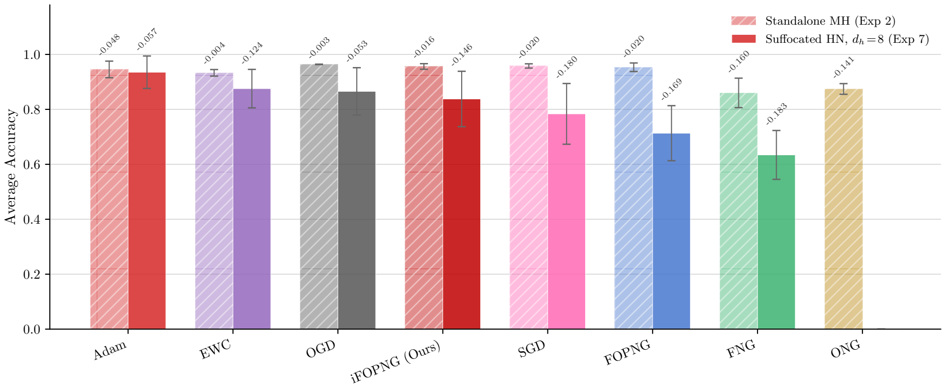
Split-MNIST — Final Average Accuracy (after Task 5)
