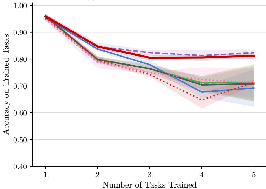
(a) Multihead CNN — Standalone
