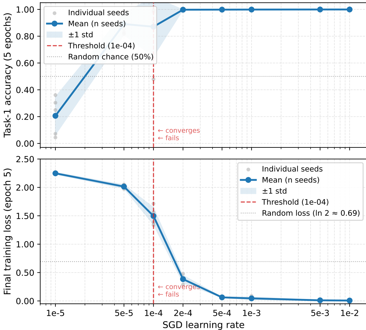
SGD convergence threshold — Split-MNIST Task-1 accuracy and loss vs learning rate (5 epochs, n seeds)
