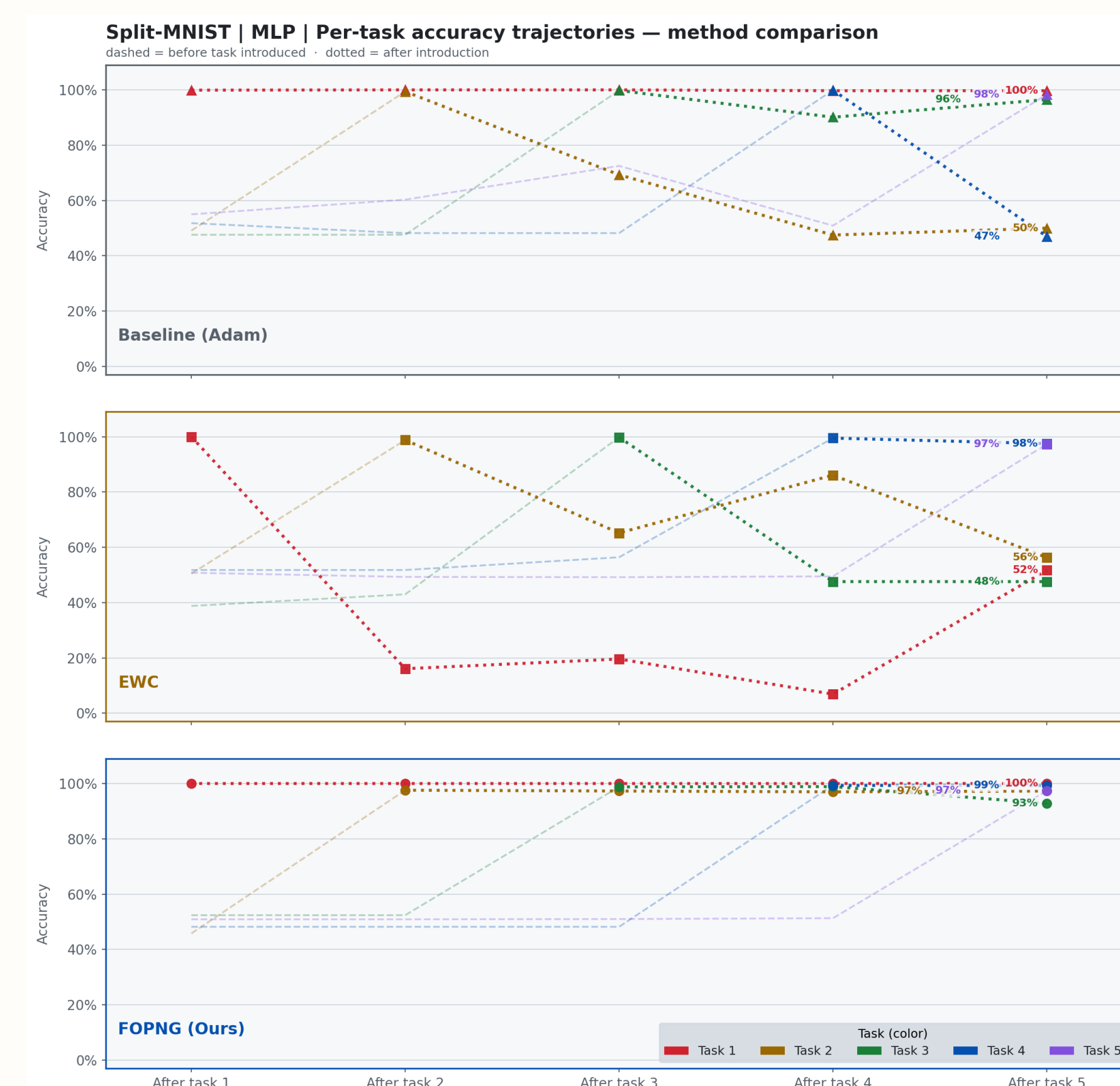
Figure 1: First preliminary results for Split-MNIST. Standard MLP performance comparison. Notice the severe performance degradation in Baseline (Adam) and partial forgetting in EWC.
