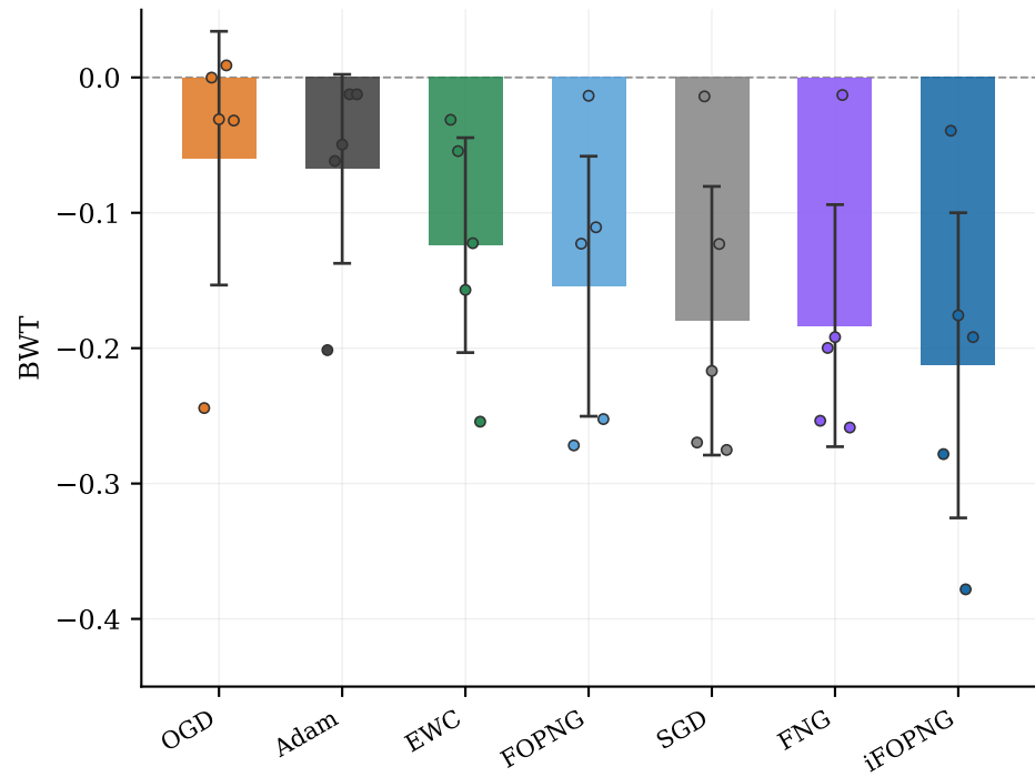
Backward Transfer
