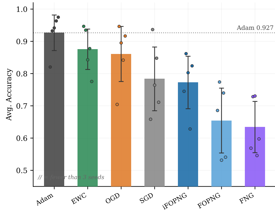
Average Accuracy
