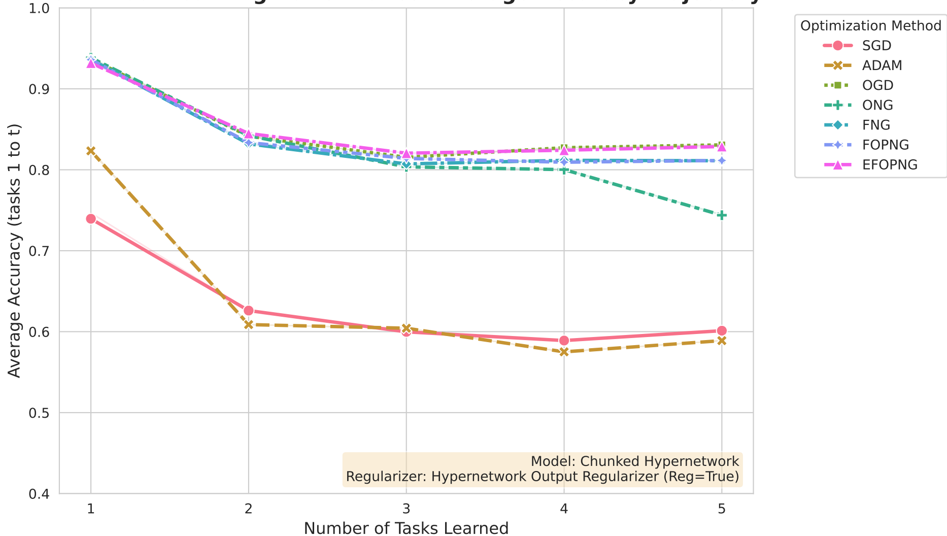
Continual Learning Performance: Average Accuracy Trajectory
