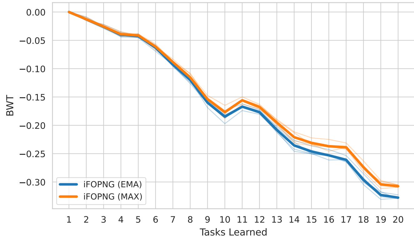
Trajectory Backward Transfer (BWT) (Thin = Seeds, Thick = Average)
