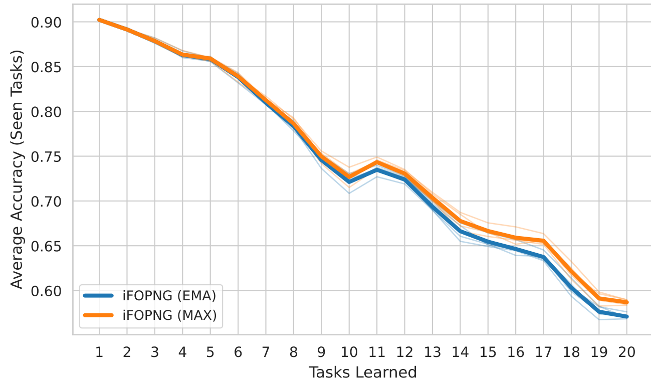
Trajectory Average Accuracy (Thin = Seeds, Thick = Average)
