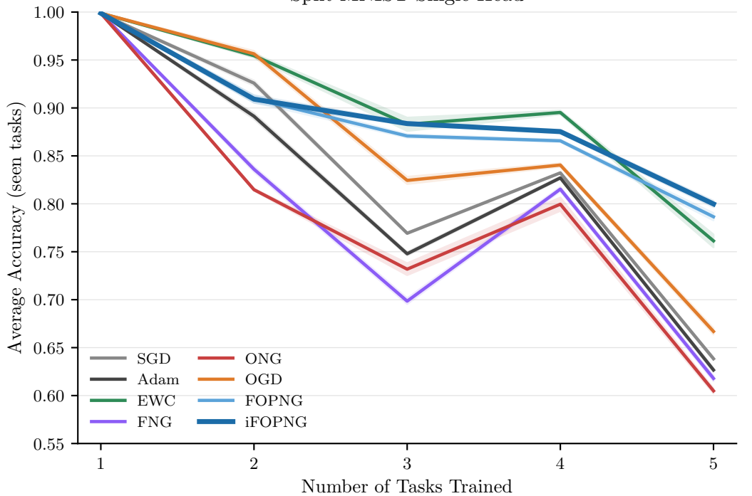
Split-MNIST Single-Head
