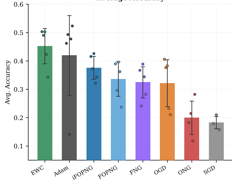
Average Accuracy
