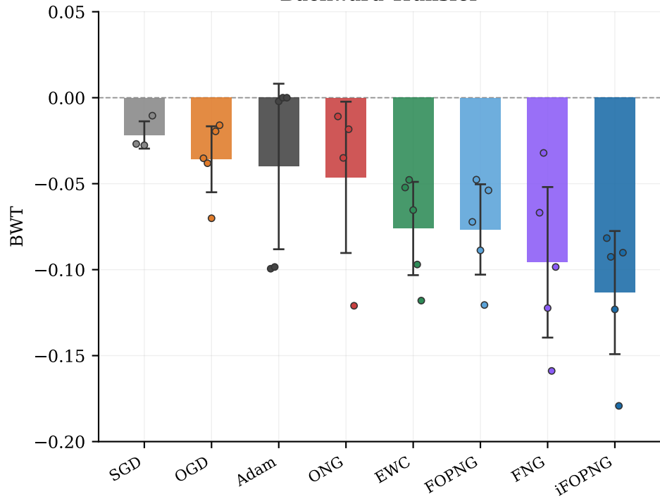
Backward Transfer
