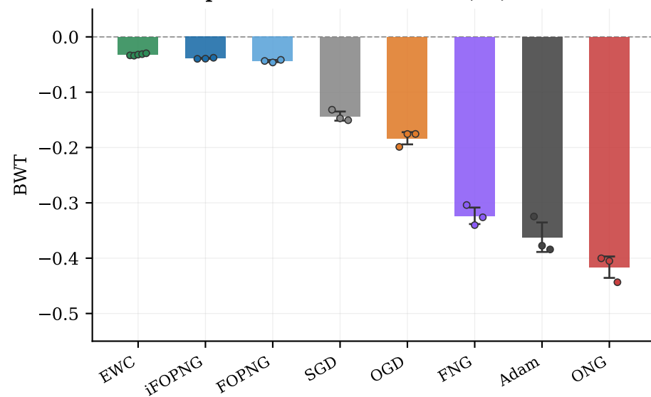
Exp 1 — Permuted-MNIST (5T) BWT
