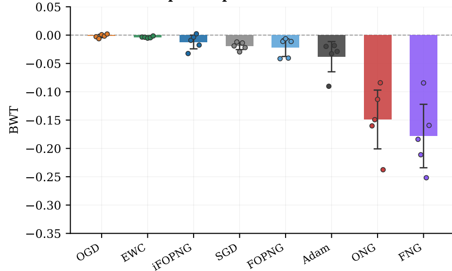
Exp 2 — Split-MNIST MH BWT
