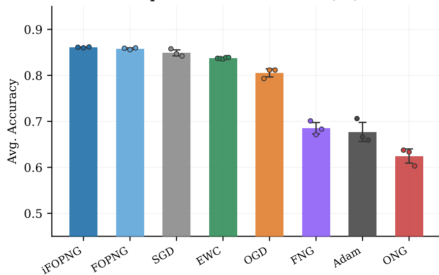
Exp 1 — Permuted-MNIST (5T)
