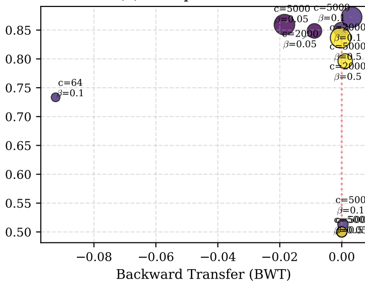
(b) Sweep B: CIFAR-10
