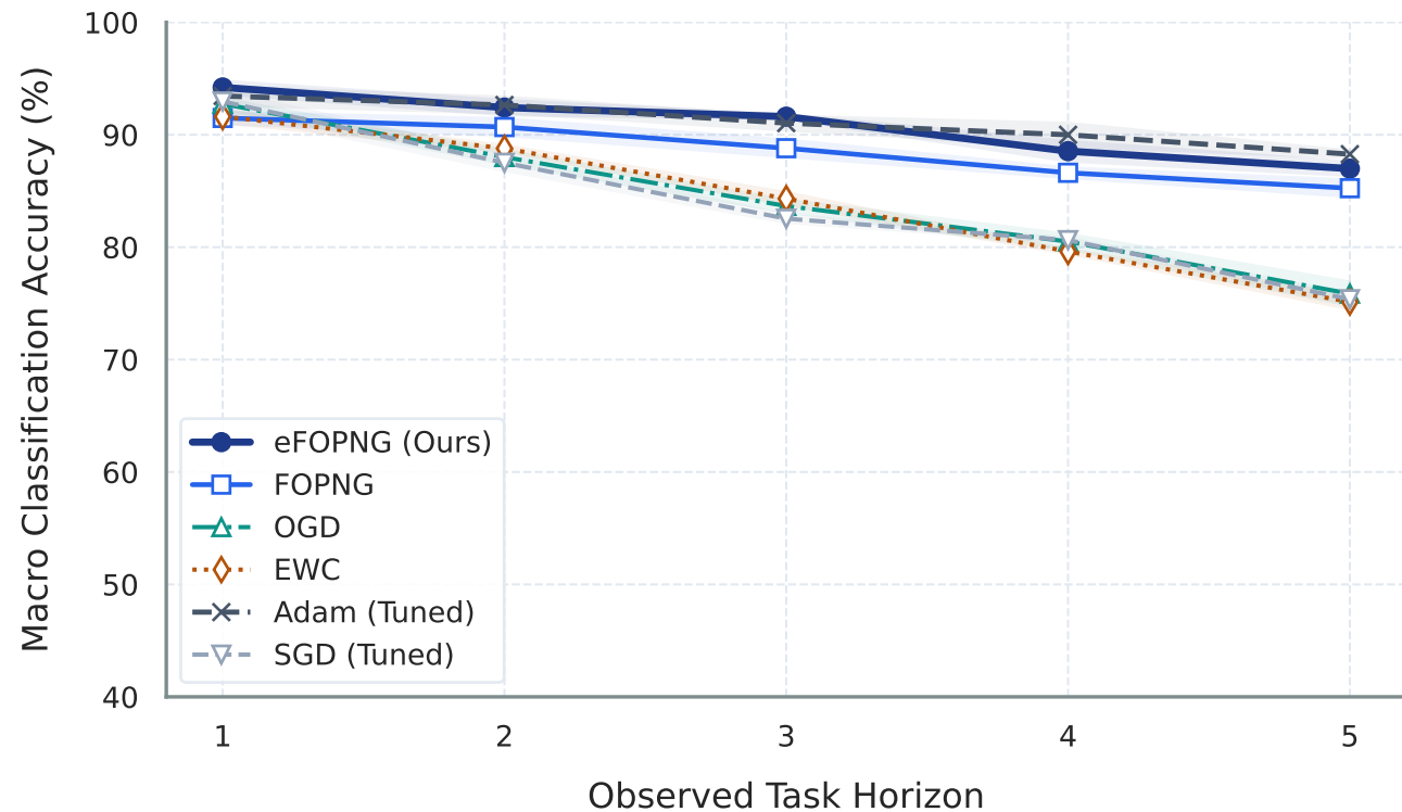
Average Accuracy Trajectory across Sequential Tasks (Split-CIFAR10)
