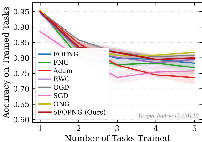
Accuracy on Trained Tasks vs Number of Tasks Trained Split-CIFAR10
