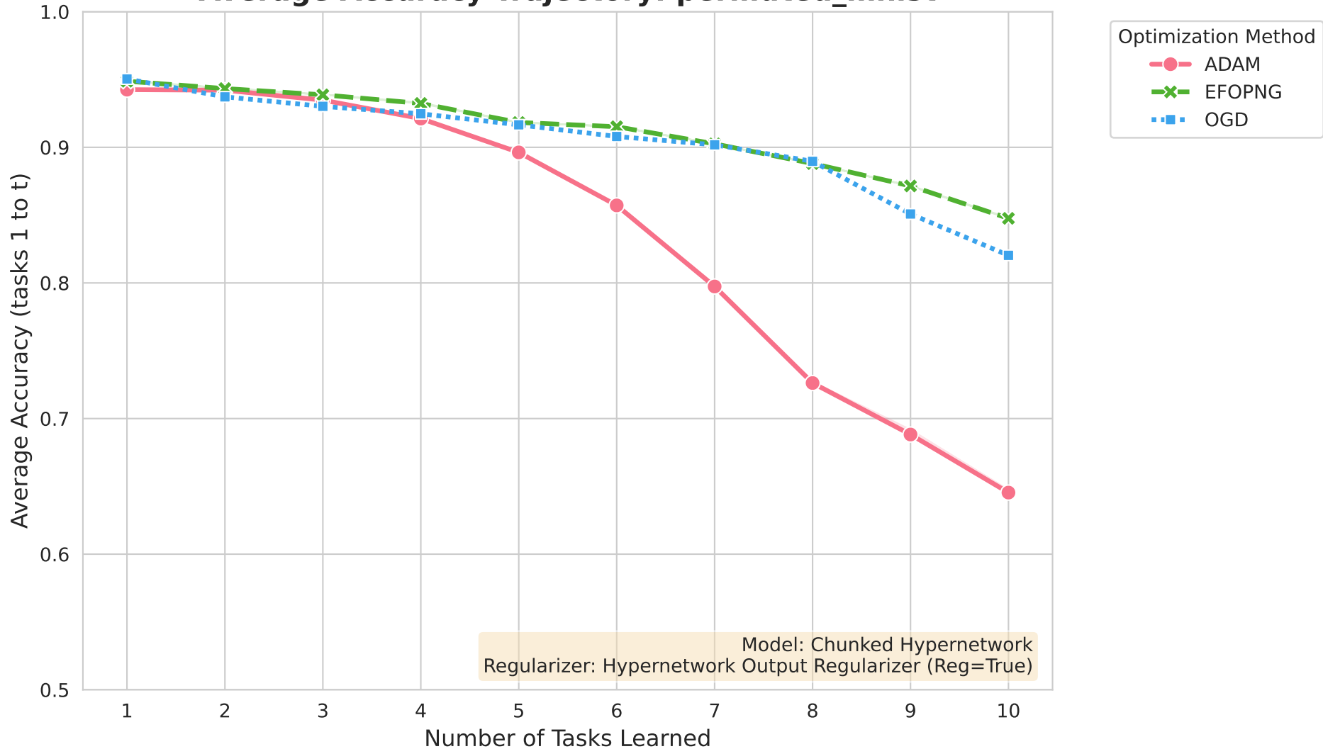
Average Accuracy Trajectory: permuted_mnist
