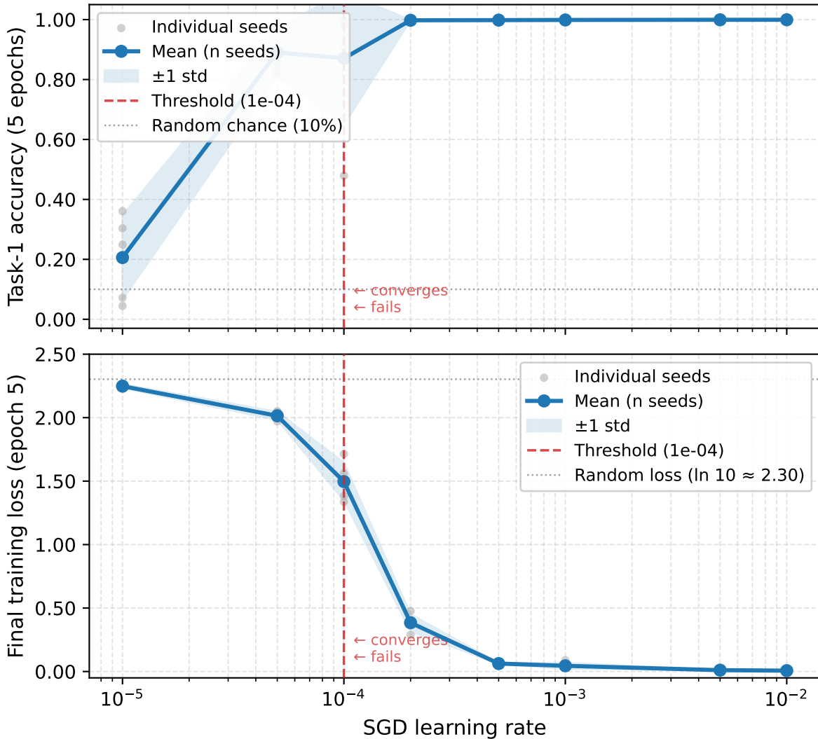
SGD convergence threshold — Split-MNIST SH Task-1 accuracy and loss vs learning rate (5 epochs, n seeds)
